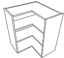
MEDIUM L-SHAPED CORNER WALL UNIT 300 x 300 opening for fascias
